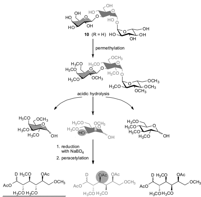
Scheme 3. Principles of linkage-type analyses using methylation and sodium deuteride reduction to alditols. Formation of their acetates and assignment by GC-MS fingerprint fragmentation (exemplary depiction for 10, R = H).
