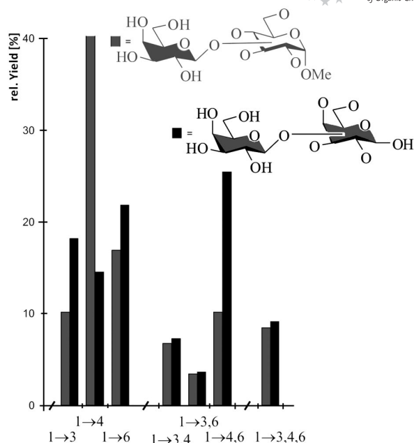
Figure 1. Results for heteromeric glycosylation couples (grey bars) and self-glycosylation of 2 (black columns).
