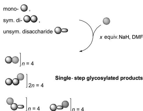
Scheme 1. Direct glycosylation of unprotected nonreducing saccharides using monosaccharide glycosides (Gal, Glc), a symmetric disaccharide ( \alpha , \alpha -trehalose) and an unsymmetric disaccharide (sucrose) as examples.
