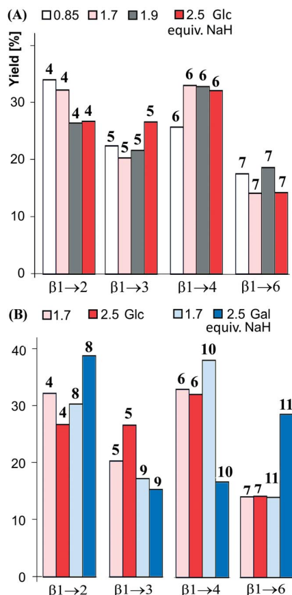
Figure 3. (A) Comparison of the relative average yield [%] at varying NaH concentrations for the four \beta Glcp-trehalose products ( 4–7 ). (B) Comparison of yields of \beta Glcp-trehaloses 4–7 and \beta Galp-trehaloses 8–11 .
