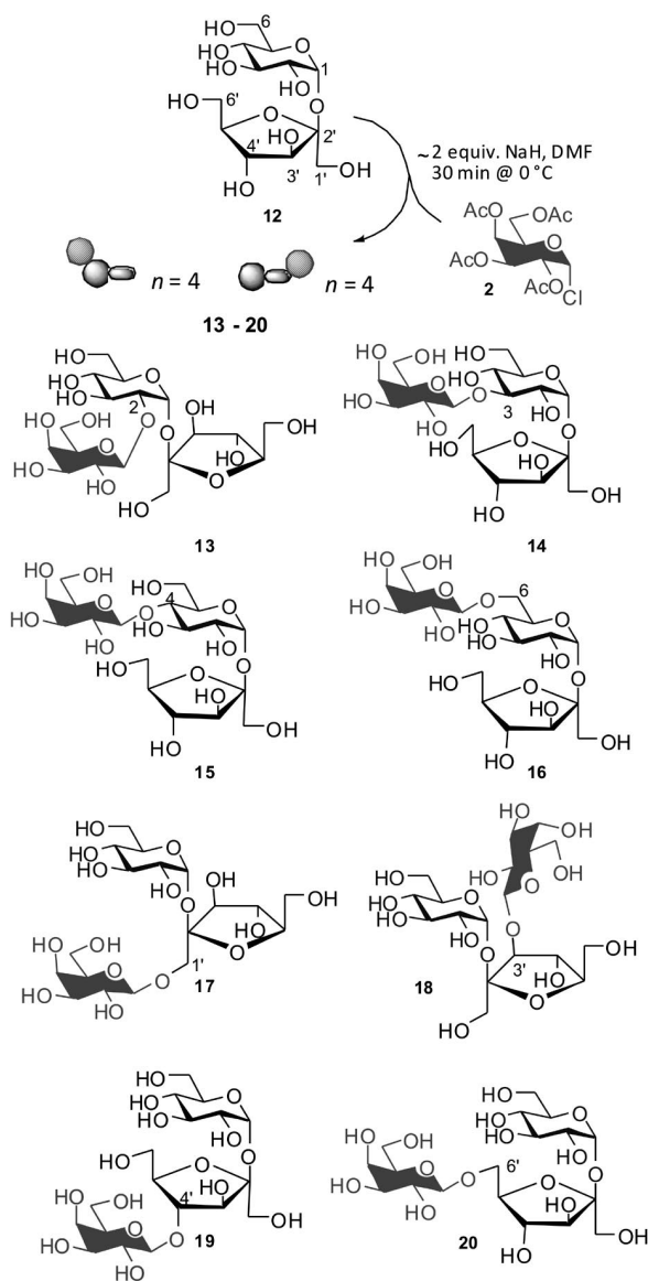
Scheme 4. Formation of galactopyranosyl sucroses 13–20.
