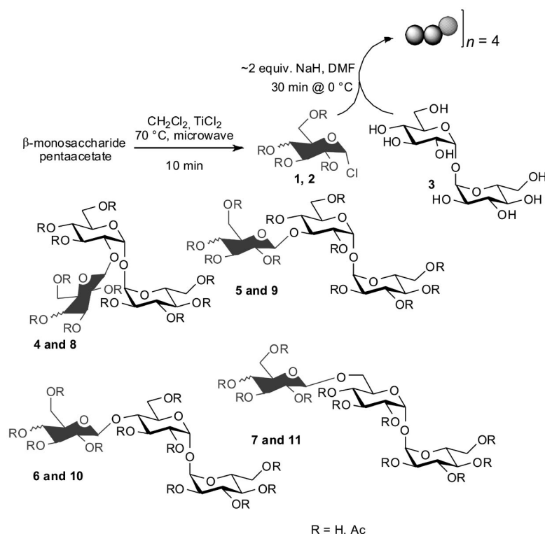
Scheme 2. Random glucosylation (series 4–7) and galactosylation (series 8–11) of \alpha,\alpha -trehalose (3).
