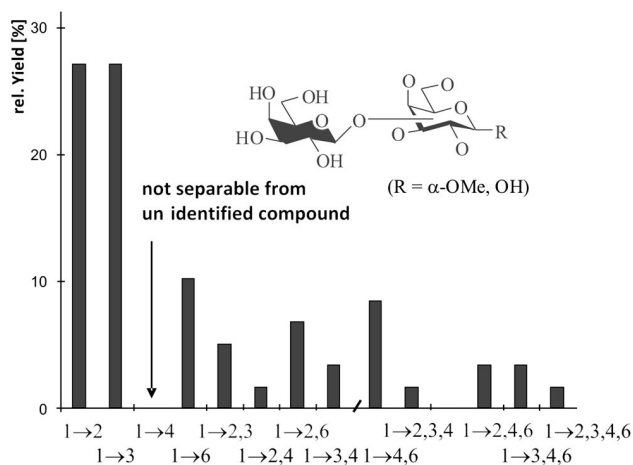
Figure 2. Result for a homomeric glycosylation of 2 .
